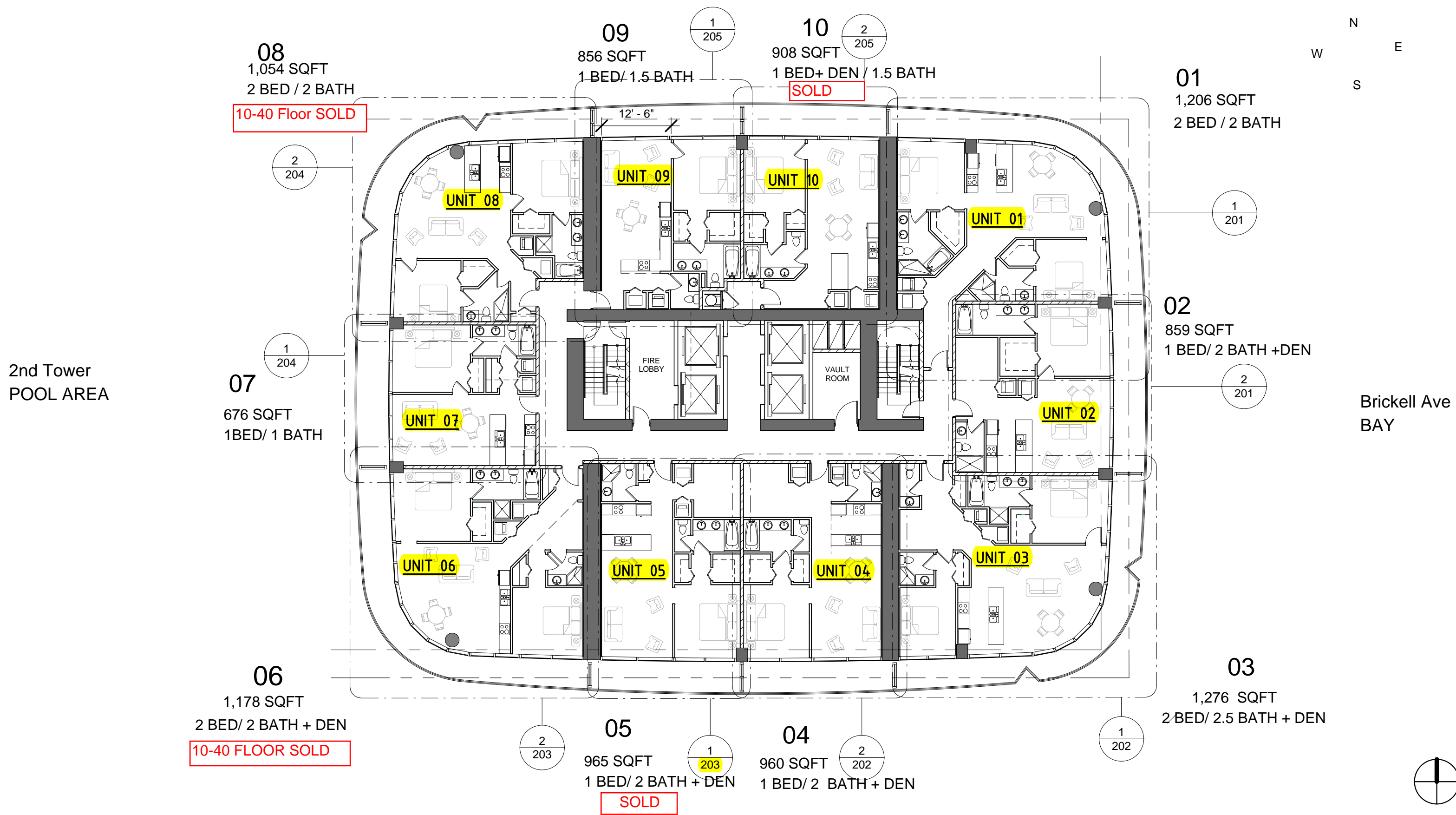
1 EAST TOWER-1ST LEVEL FLOOR PLAN 1/16" = 1'-0"
